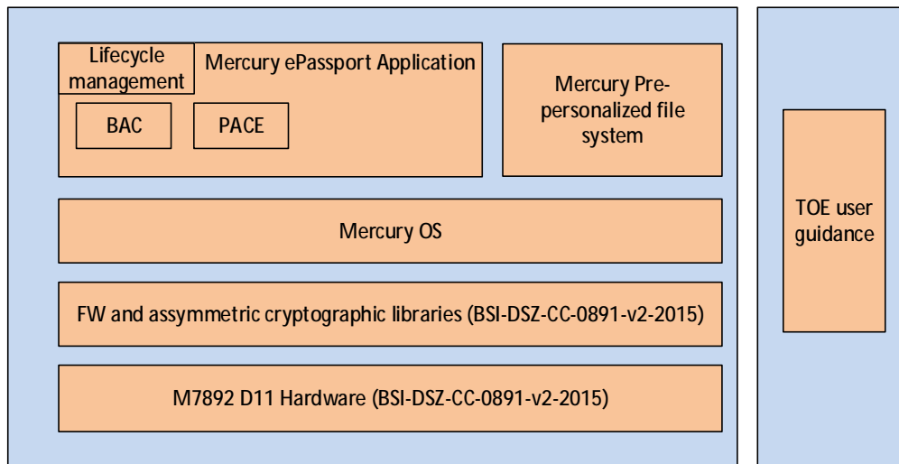
Figure 1. Logical architecture of the TOE.
