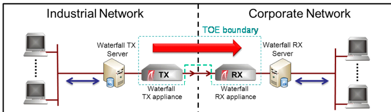
Figure 1-1 – Typical Usage Scenario
