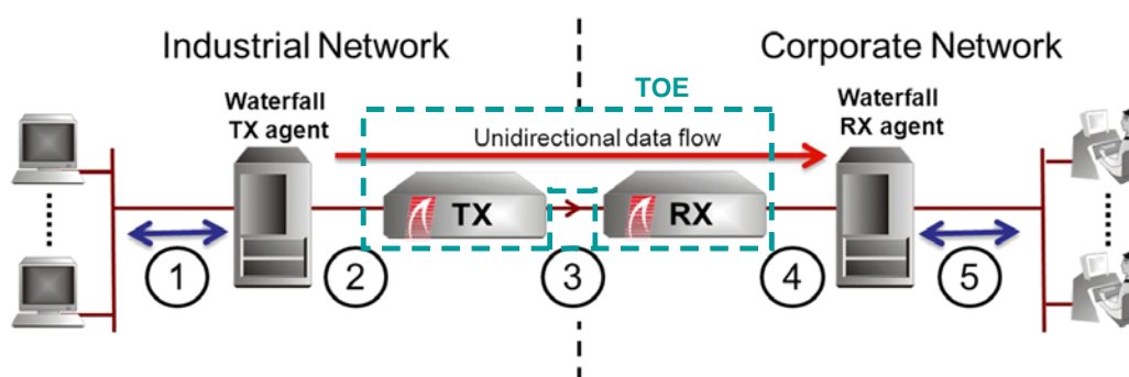
Figure 1-3 –Information Flow through the TOE
