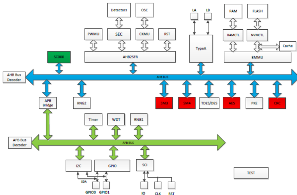
Figure 1. Hardware Blocks of the TOE (the security-no-claimed parts are marked red).
