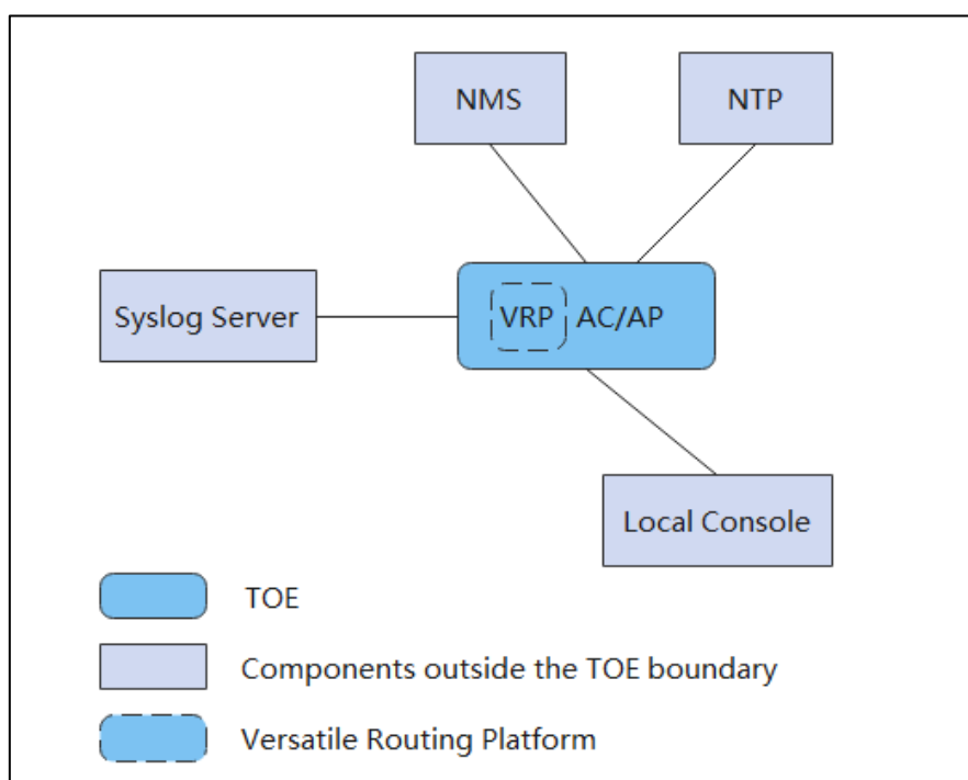
Figure 1-1 IT Entities which connect with TOE
